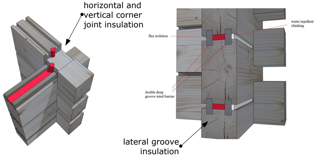
3RADI log wall with massive stud corner joint (wall do not settles at all)
